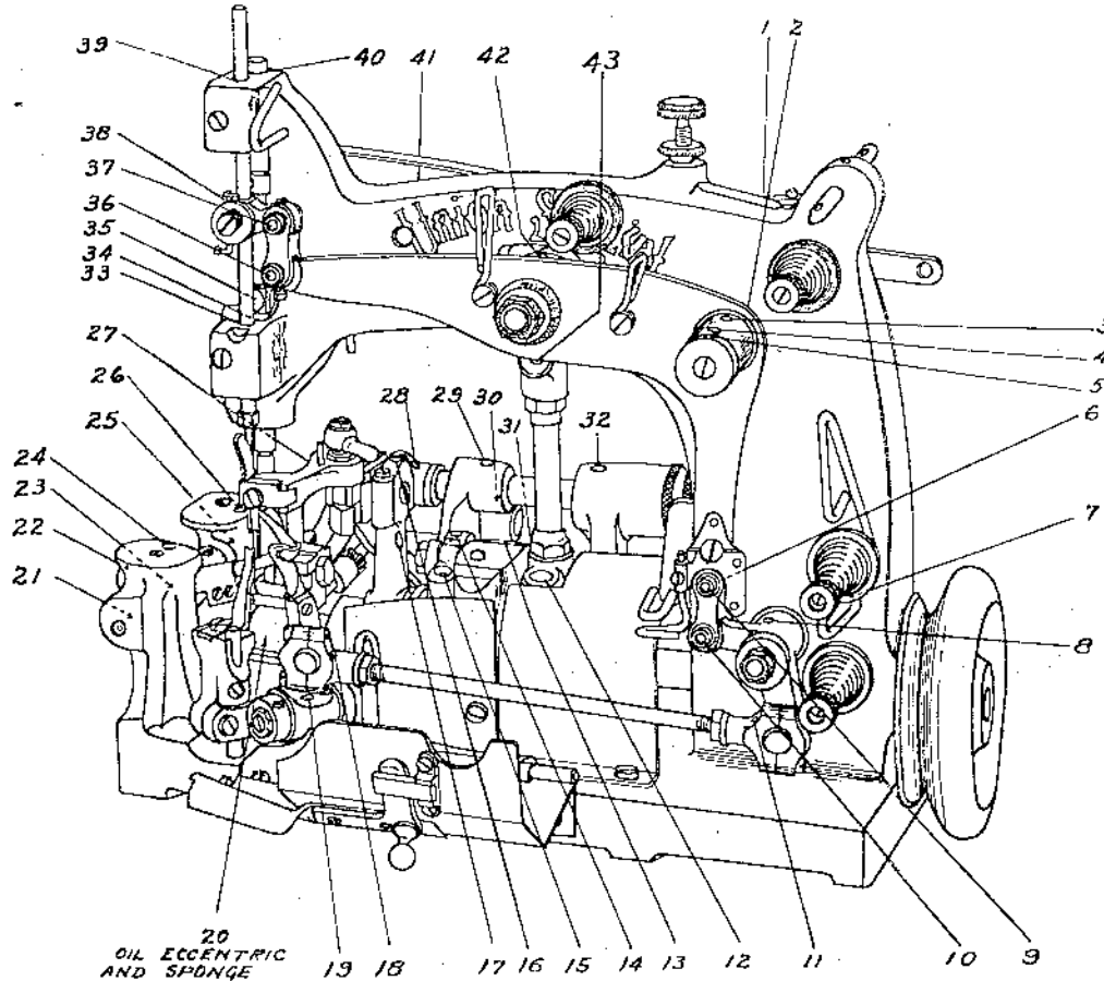
CLASS 15400 Machine
