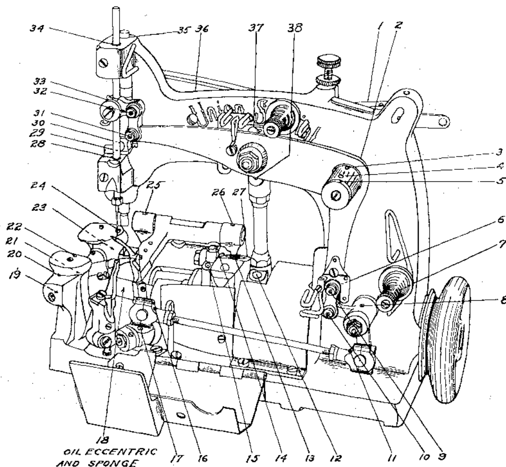
CLASS 15500 Machine
